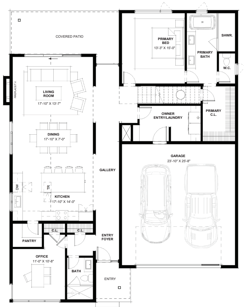
MAIN FLOOR
